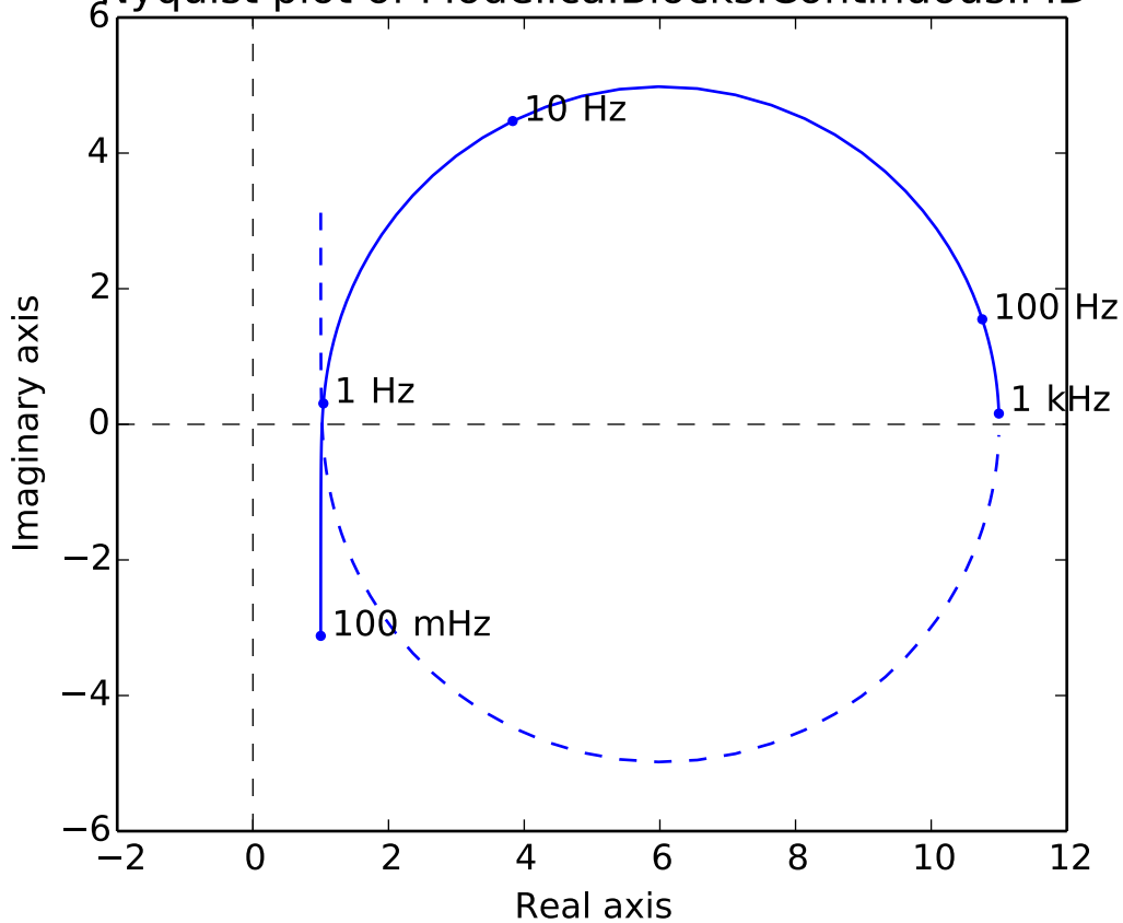
Nyquist plot of Modelica.Blocks.Continuous.PID
